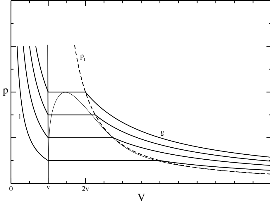
Figure 2: Schematic representation of the gas-liquid isotherms (curves g and, respectively, l ), with the critical region indicated by the cutoff volume v to 2v . The coexistence curve p_t is given by equation (22).
