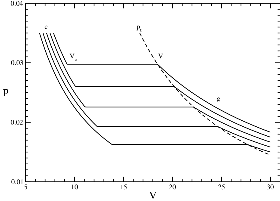
Figure 1: Gas-condensate isotherms p = NT/V (gas, curves g ), p = NT/sV (condensate, curves c ) and the transition (coexistence) curve p_t given by p_t = NT_t/V = sN\varepsilon_0/(s-1)V \ln(V/v) according to equation (22) for sN\varepsilon_0/(s-1) = 1 , (s-1)T/s\varepsilon_0 = 0.450, 0.475, \dots, 0.550 (step 0.025), v = 3 and s = 2 . The hs coexistence curve is pushed in fact toward a limiting volume v (not shown in figure), as discussed in text and shown in Fig. 2.
