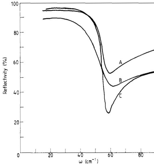
Figure 2. Theoretical reflectivity at normal incidence (22) for two values of the phason lifetime \Gamma_\phi^{-1} compared with the experimental one (Brüesch et al 1975). The following values of the parameters are used: \omega_T = 1.9 \text{ meV} , \tilde{\Delta} = 100 \text{ meV} (Brüesch et al 1975) and \omega_p = 2.88 \text{ eV} (Kuse and Zeller 1971). The electron-phonon coupling strength is taken to be \lambda = 0.45 but the reflectivity is slightly dependent on \lambda in the range 0.37–0.49 of the most reliable values (see table 1 and discussion therein). The CDW plasma edge \omega_L at about 56 \text{ cm}^{-1} (7 meV) is in excellent agreement with the experimental value. The curves are: A, experiment; B, \Gamma = 1.0 \text{ meV} ; C, \Gamma = 0.3 \text{ meV} .
