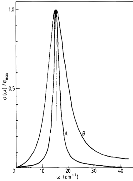
Figure 1. Normalised far-infrared conductivity, \sigma(\omega)/\sigma_{\max} , given by (21) compared with the experimental one (Brüesch et al 1975) for \omega_T = 15 \text{ cm}^{-1} (1.9 meV). A, \Gamma = 0.3 \text{ meV} ; B, experiment.
