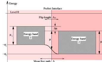
Fig.3. Two Solids with a Perfect Contact
