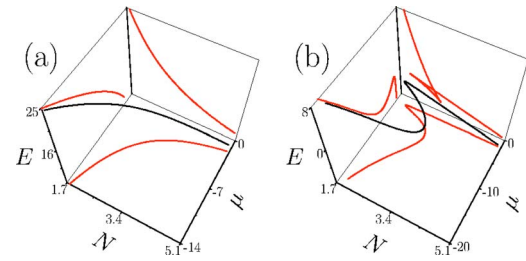
FIG. 2. (Color online) The soliton family in terms of the dependence E = E(\mu, N) , and its projections on the planes (E, \mu) , (E, N) , and (\mu, N) for (a) p=0 and (b) p=3 .
