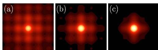
FIG. 4. (Color online) Integrated through views along the z axis of the solitons shown in Fig. 3.
