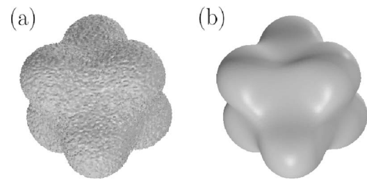
FIG. 5. Isosurface plots showing self-cleaning of a stable soliton corresponding to p=3 and N=2.4 , initially perturbed by white noise. (a) Input at t=0 ; (b) output at t=50 .
