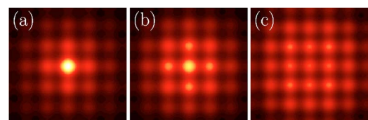
FIG. 6. (Color online) Integrated through views along the z axis of an unstable soliton that decays due to a uniform norm-reducing perturbation with \epsilon=0.01 , for p=3 . (a) t=0 , A=1.78 ; (b) t=50 , A=0.6505 ; (c) t=70 , A=0.2075 .
