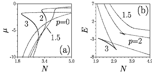
FIG. 1. The chemical potential \mu (a) and the energy E (b) of the 3D solitons vs their norm N for different values of the lattice strength p . Full and dotted lines depict stable and unstable solitons, respectively.
