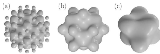
FIG. 3. Isosurface plots of (a) unstable and (b and c) stable 3D solitons. Here p=3 ; (a) N=2.4 , A=1.8 , (b) N=2.04 , A=2.2 , and (c) N=2.4 , A=3 .
